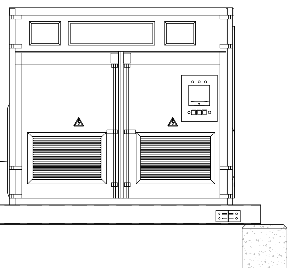
Inverter Container
