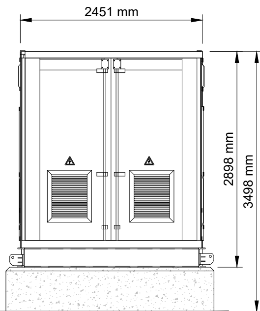
Inverter Container
