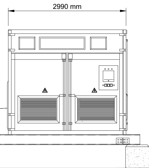
Inverter Container
